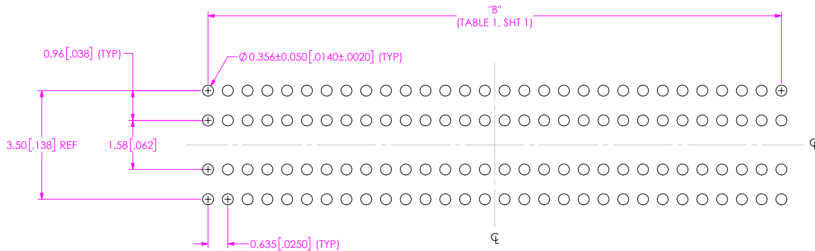
FIG 2 ADF6-30-XX.X-XXX-4-X-A STENCIL SHOWN
