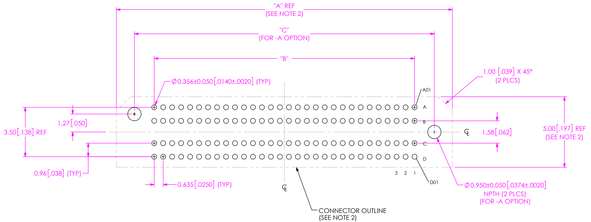
FIG 1 ADM6-30-XX.X-XXX-4-X-A FOOTPRINT SHOWN
