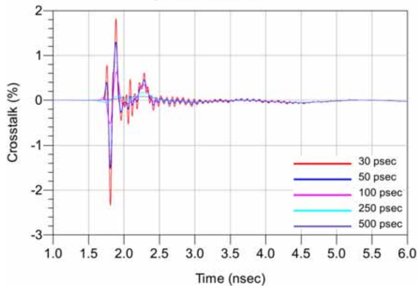
Single-Ended Application - FEXT
