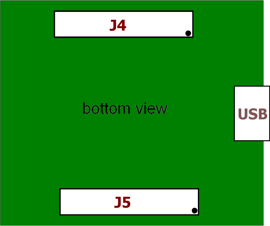
Connector receptacles J4 and J5 (bottom view)
