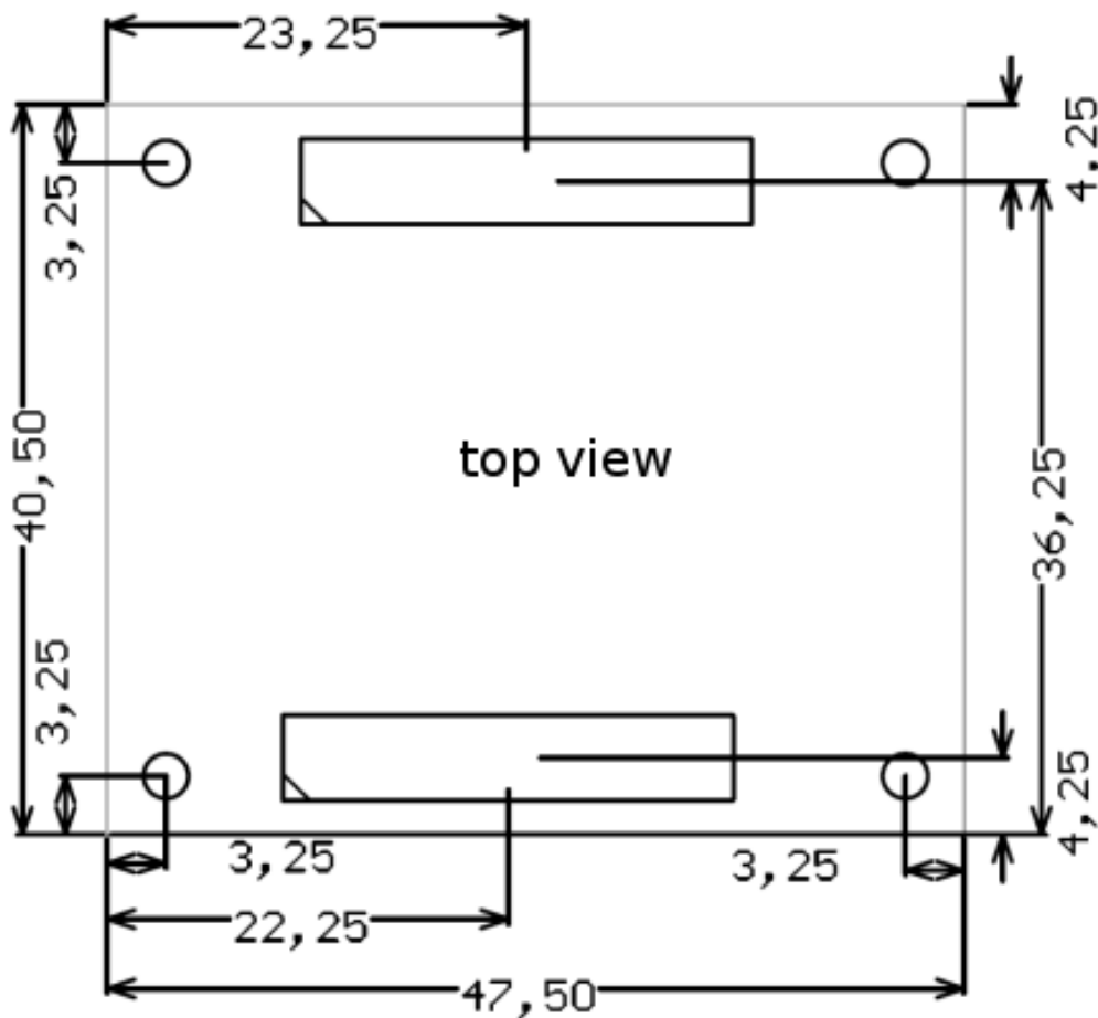
Dimensional drawing, TE0630 measures 40.50 x 47.50 mm.
