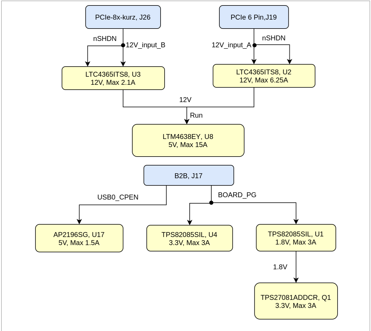
Power Sequence
