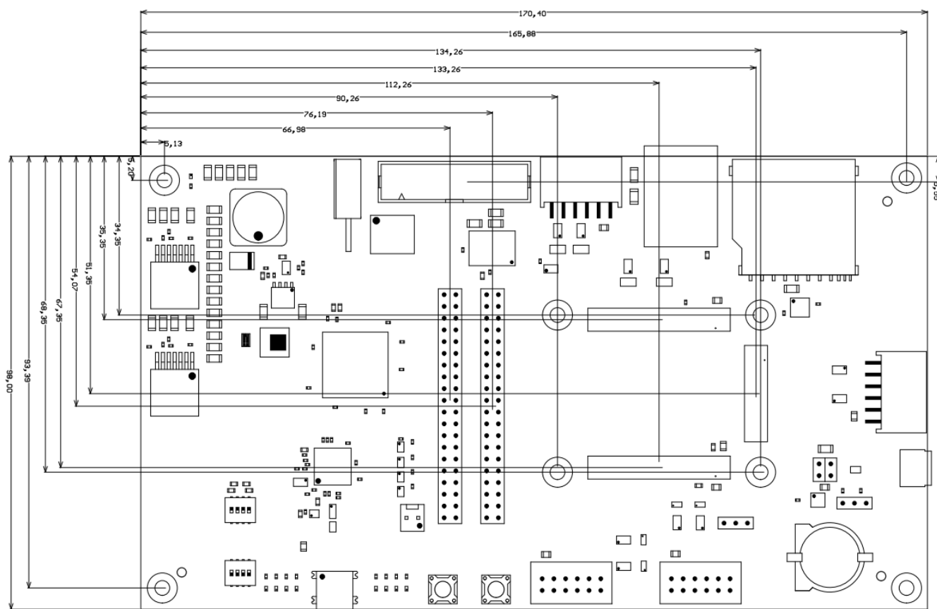
Figure 4: Physical dimensions of the TE0705-04 carrier board.
