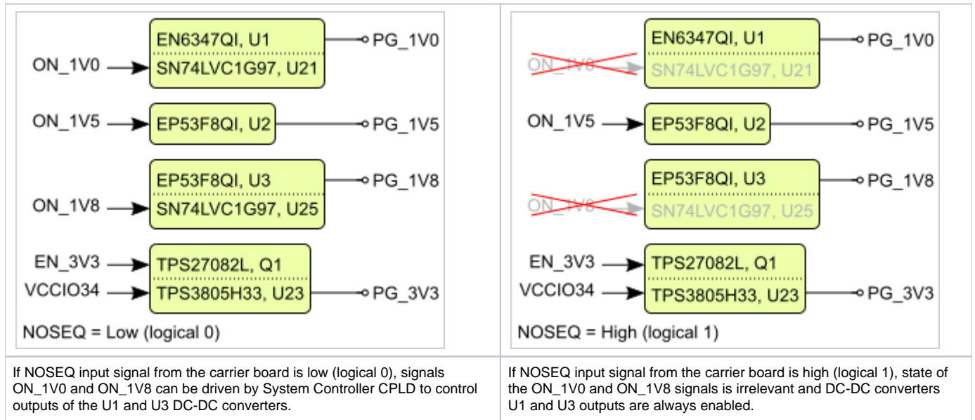
Figure 4: Power sequencing.
