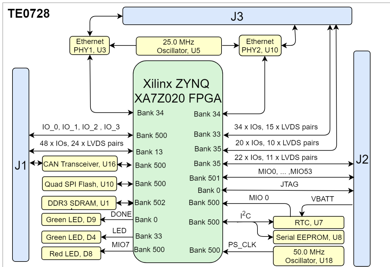
TE0728 block diagram
