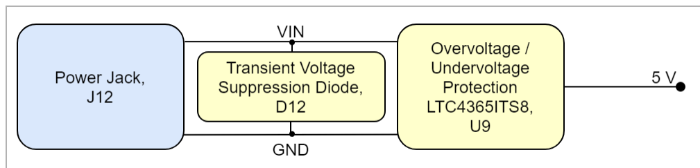
Voltage Protection Circuit
