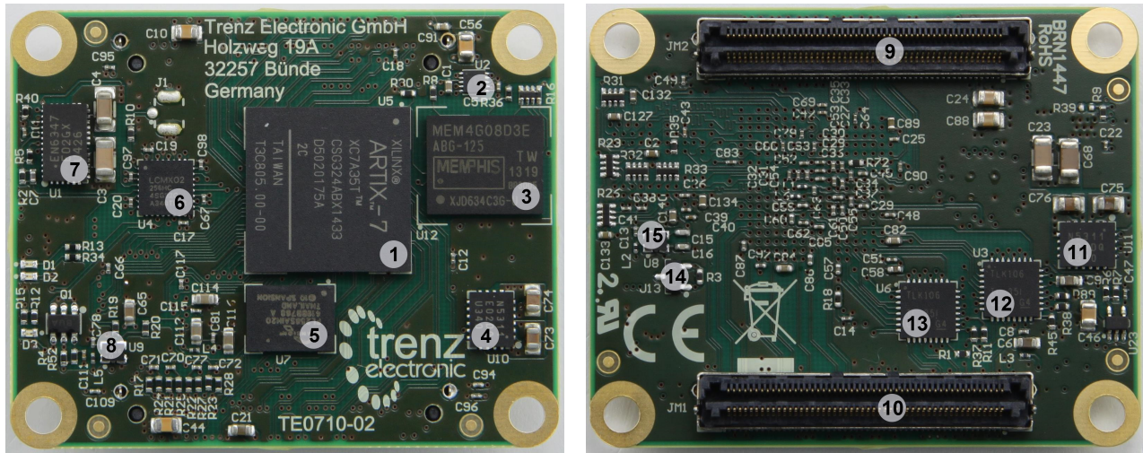
Figure 2: TE0710-02 PCB.
