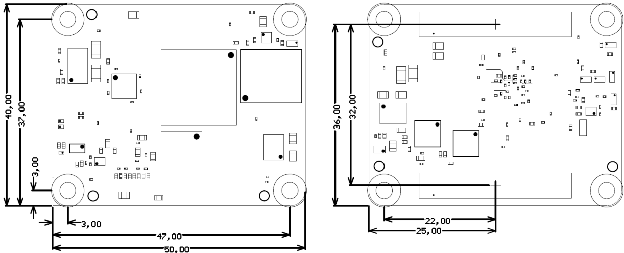
Figure 3: Physical dimensions of the TE0710-02 SoM.
