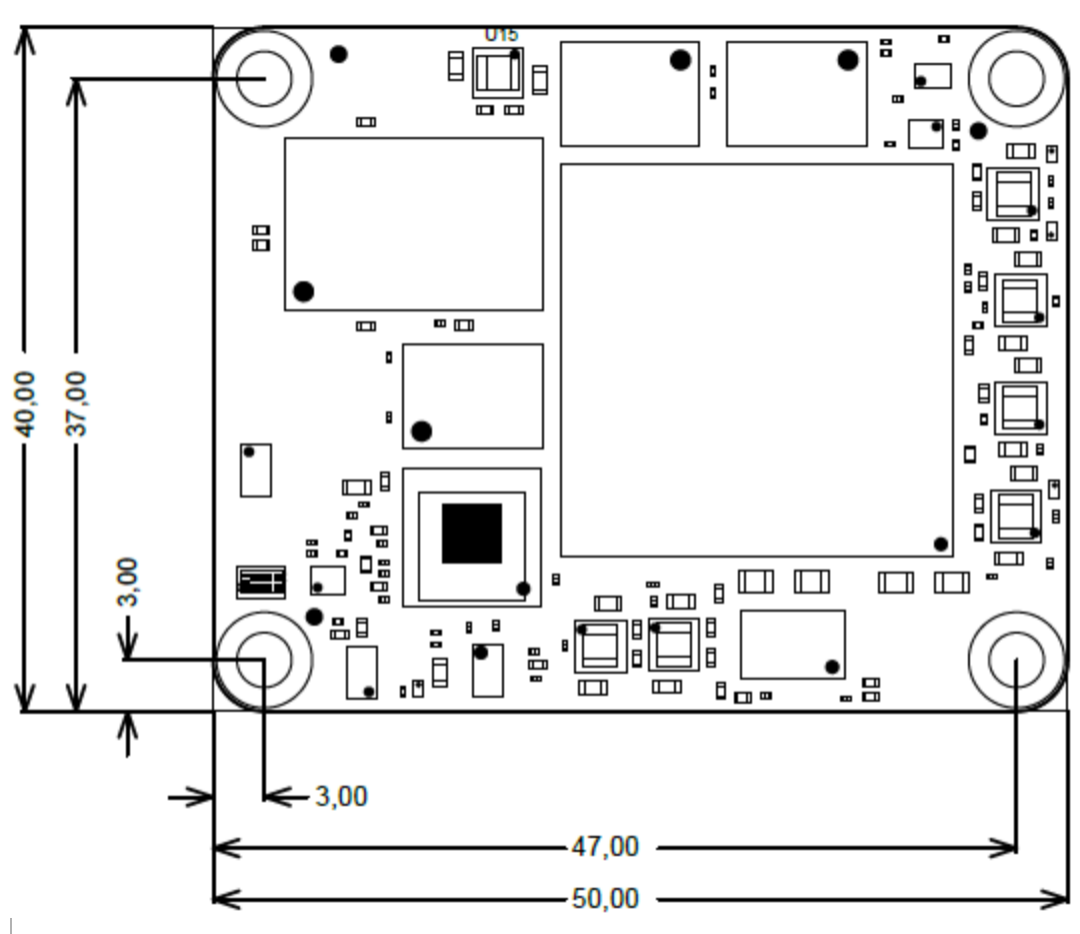
Physical Dimension
